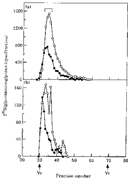
FIG. 5. Sephacryl S-200 chromatography of newly synthesized [ 35 S]-sulfated glycosaminoglycans. Pooled proteoglycan fractions were digested with papain and applied to Sephacryl S-200 columns. [ 35 S]-Sulfated glycosaminoglycans from control (open circles) and PEMF-treated (solid circles) cultures were eluted at room temperature with 0.5 M sodium acetate, pH 7.0, at a rate of 1.5 ml/h. Fractions were analyzed for radioactivity. V_0 and V_t indicate the void volume and the total bed volume of the columns, respectively. (a): extract, (b): medium.
