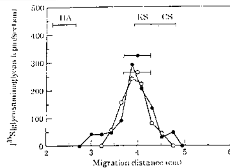
FIG. 10. Cellulose acetate electrophoresis of newly synthesized [^{35}\text{S}] -sulfated glycosaminoglycans. Pooled glycosaminoglycan fractions were dialysed, lyophilized and subjected to electrophoresis. Samples from control (open circles) and PEMF-treated (solid circles) cultures were run on cellulose acetate strips in 0.1 M \text{KH}_2\text{PO}_4 , 0.1 M HCl, pH 2.0, with a potential gradient of 5 V/cm for 3 h. Hyaluronic acid, chondroitin sulfate and keratan sulfate were included as standards. Strips were either stained with alcian blue, denoted by the bars, or sectioned and analyzed for radioactivity.
