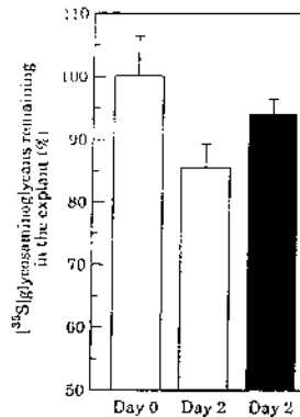
FIG. 7. Degradation of pre-existing [ 35 S]-sulfated glycosaminoglycans in explant cultures. Sterna were isolated from embryos previously administered with [ 35 S]sulfuric acid in ovo . The fate of the pre-existing [ 35 S]-sulfated glycosaminoglycans after 2 days culture in the absence (hatched column) or presence (solid column) of PEMF was determined and expressed as percentage of radioactivity retained by the explant. All data are the means \pm s.d. of at least three measurements.
